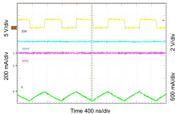
Figure 10-29. Light Load Operation Showing SW
