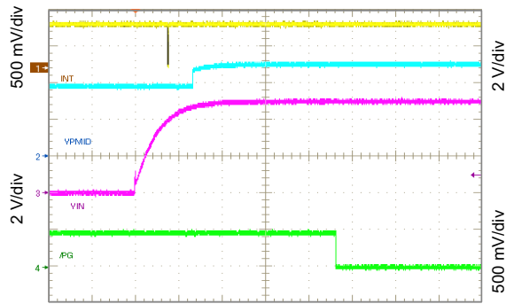
Time 10 ms/div Figure 10-59. Show PG and INT Timing (VIN Insertion)
