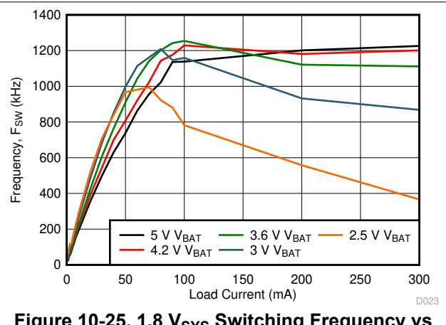
Figure 10-25. 1.8 V sys Switching Frequency vs Load Current
