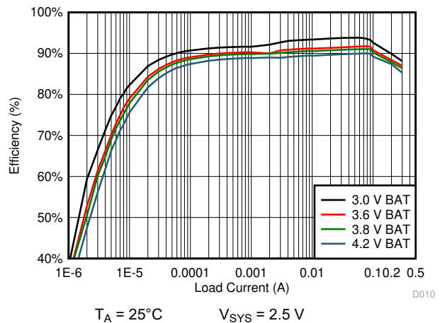
Figure 10-13. 2.5 V SYS System Efficiency
