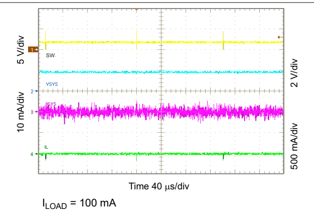
Figure 10-27. Light Load Operation Showing SW
