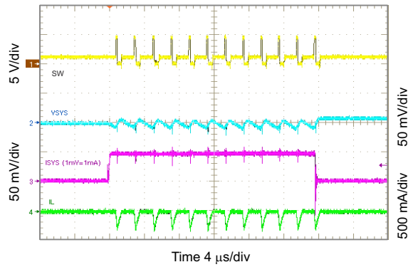
Figure 10-33. 1.2 V sys Load Transient, 0 to 50 mA
