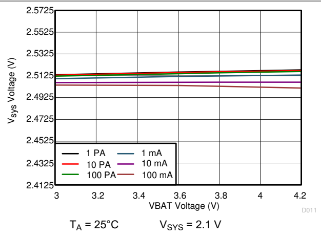
Figure 10-23. 2.1 V sys Line Regulation
