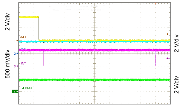
Time 400 μs/div Figure 10-62. PG Functions as Shifted MR Output
