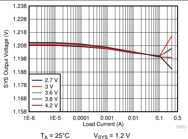
Figure 10-15. 1.2 V SYS Load Regulation
