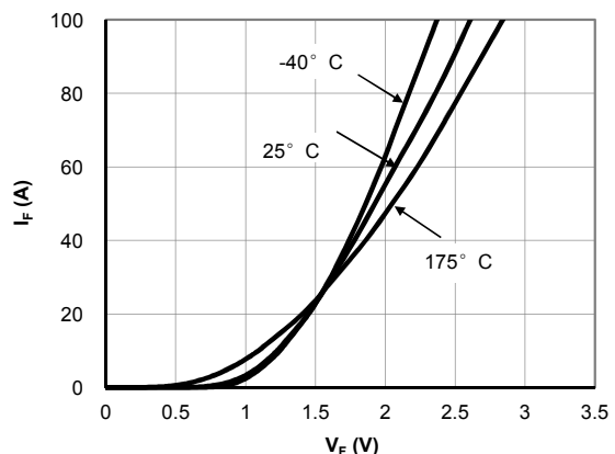
Figure 4: Diode Characteristic
