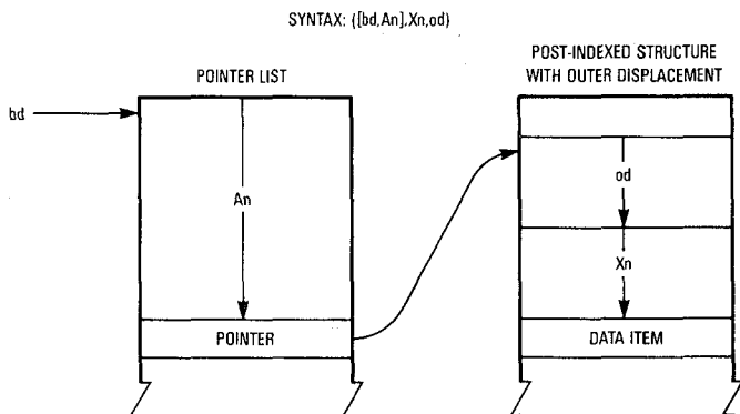
Figure 2-14. Postindexed Indirect Addressing with Outer Displacement
