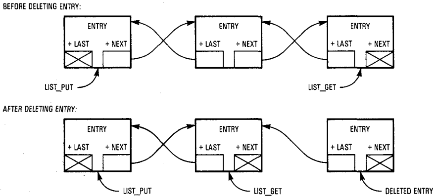
Figure 3-5. Doubly Linked List Deletion
