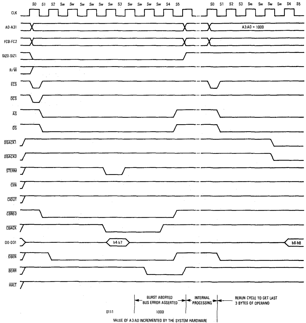
Figure 7-53. Long-Word Operand Request — \overline{BERR} on Second Access
