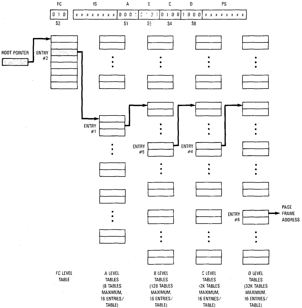
Figure 9-20. Five-Level Table Search
