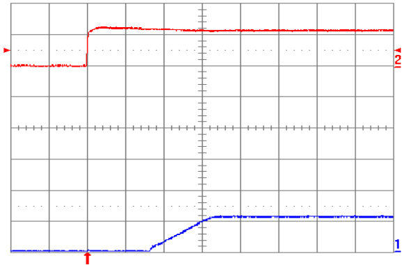
Fig. 1.2V.4: Turn-on transient for V_{out} = 1.2V with application of V_{in} at full rated load current (resistive) and 100\mu F external capacitance at V_{in} = 12V . Top trace: V_{in} (10V/div); Bottom trace: output voltage (1V/div); Time scale: 2ms/div.
