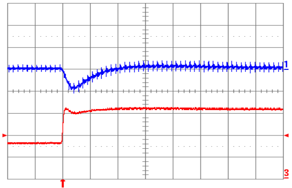
Fig. 0.7525V.6: Output voltage response for V_{out} = 0.7525V to positive load current step change from 8A to 16A with slew rate of 5A/\mu s at V_{in} = 12V . Top trace: output voltage (20mV/div.); Bottom trace: load current (5A/div.). C_o = 100\mu F ceramic. Time scale: 20 \mu s /div.
