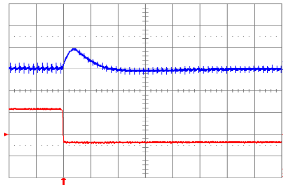
Fig. 0.7525V.7: Output voltage response for V_{out} = 0.7525V to negative load current step change from 16A to 8A with slew rate of -5A/\mu s at V_{in} = 12V . Top trace: output voltage (20mV/div.); Bottom trace: load current (5A/div.). C_o = 100\mu F ceramic. Time scale: 20 \mu s /div.
