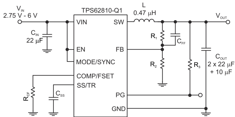
Figure 10-1. Typical Application
