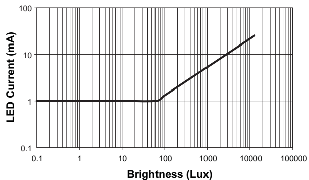
Figure 28: Backlight LED Current vs. Light Brightness.
