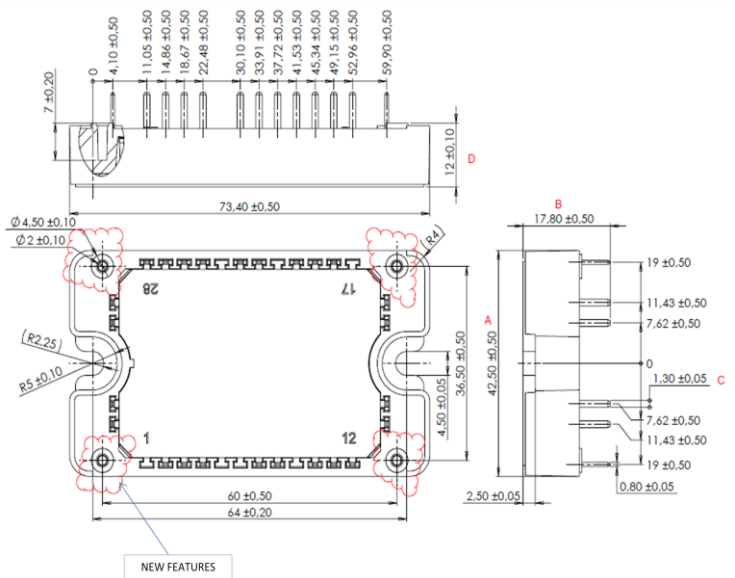
SP3F plastic frame
