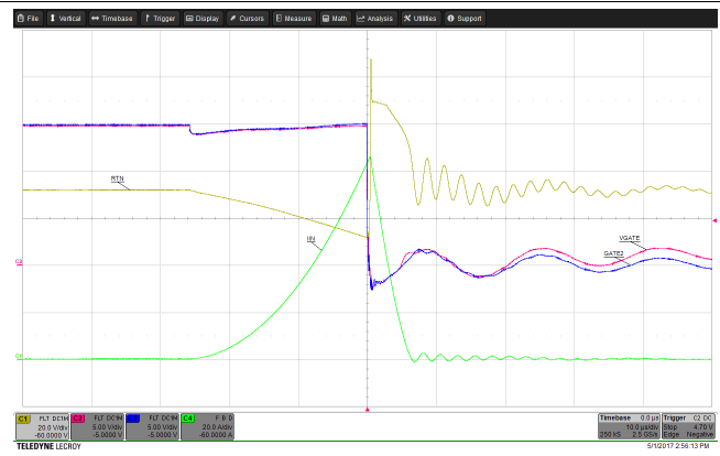
Figure 20. Hot Short (Vin = 72 V, no load)
