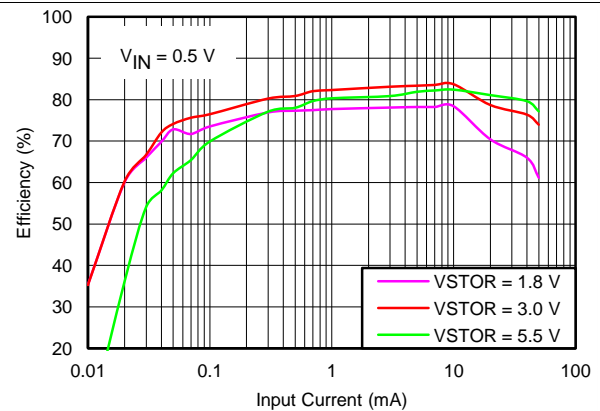
V_{IN\_DC} = sourcemeter configured with voltage source = 0.5 V and I_{COMP} varied from 0.01 mA to 100 mA V_{STOR} = sourcemeter configured to measure current and voltage source set to hold the V_{STOR} voltage = 1.8 V, 3.0 V or 5.5 V
