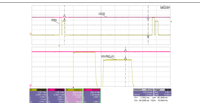
V_{IN\_DC} = sourcemeeter with V_{SOURCE} = 2.0\text{ V} and compliance of 43\text{ mA} V_{BAT} = sourcemeeter with V_{SOURCE} = 3.6\text{ V} and compliance of 1\text{ A}
