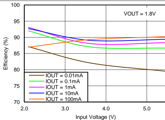
VSTOR = sourcemeter configured as a voltage source, measuring current OUT = sourcemeter configured sink current with VCOMP>V(OUT)
