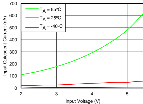
VIN_DC = floating and \overline{EN} = VSTOR VSTOR = sourcemeter configured to measure current and voltage source varied from 2.0 V or 5.5 V
