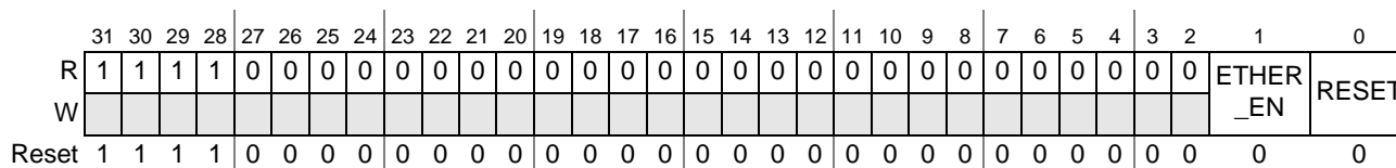
Figure 17-6. Ethernet Control Register (ECR)
