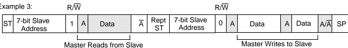
Figure 24-11. Data Transfer, Combined Format
